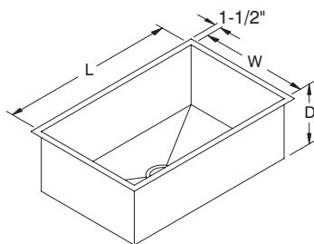
Inside Sink Bowl Dimensions
